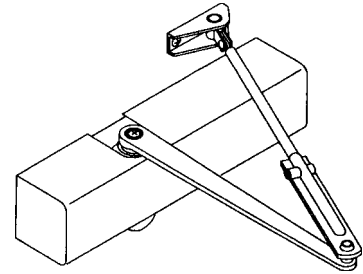
Parallel Arm Mounting
